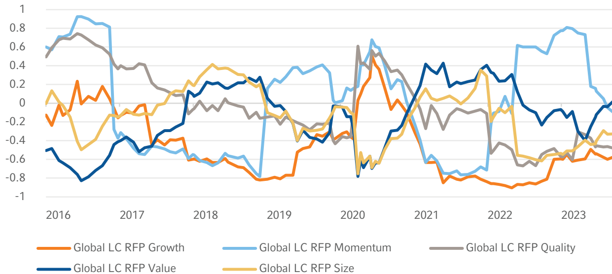
Figure 5: Ex-ante correlations with Global LC Low Volatility RFP (01/2016–09/2023)
