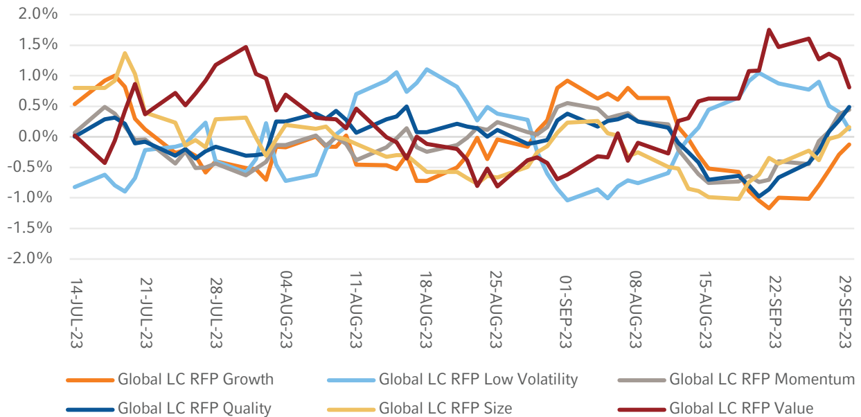
Figure 2: 10-Day rolling excess returns for Global RFPs vs. MSCI ACWI (07/03/2023–09/30/2023)
