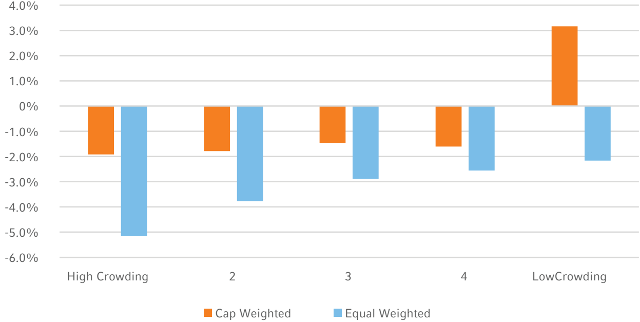
Figure 7: Annualized excess returns of the crowding factor vs MSCI ACWI
